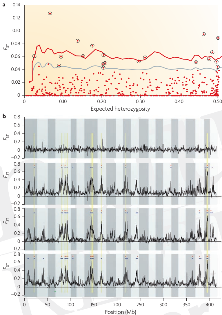
Genome scans for selection can focus on either candidate loci or anonymous loci. Namroud et al. 62 sampled white spruce ( Picea glauca ) from 6 populations in Quebec and genotyped 534 SNPs located on 345 candidate genes. Part a of the figure shows their F_{ST} outlier analysis of these data, based on the relationship between F_{ST} and expected heterozygosity 59 ; the grey and red lines represent the 95% and 99% confidence levels, respectively. Against a background of little population differentiation ( F_{ST} = 0.006 ), this analysis identified 20 SNPs (circled dots) in 19 genes above the 95% confidence level. New genomic tools also allow anonymous markers to be assayed across the genome to identify local adaptation; for example, Hohenlohe et al. 66 sampled 100 threespine stickleback individuals across 5 populations in Alaska. They used sequencing of restriction-site-associated DNA (RAD) tags 127 to simultaneously identify and genotype over 45,000 SNPs across the genome. This density of markers allows population genetic statistics, such as F_{ST} , to be visualized as continuous distributions along chromosomes. In part b of the figure, the top panel shows F_{ST} between the two marine populations. The next three panels show differentiation between each of the three freshwater populations and the two marine populations. Coloured bars above each graph show regions of significantly elevated F_{ST} as indicated by bootstrap resampling (blue, p \leq 10^{-5} ; red, p \leq 10^{-7} ). Vertical grey shading indicates the chromosomes, and yellow shading indicates the nine most significant and consistent peaks of freshwater-versus-marine differentiation. Common patterns of population differentiation (yellow shading shared among the three populations) indicate genomic regions that have responded to divergent selection in parallel across populations. The image in part a is reproduced, with permission, from REF. 62 © John Wiley and Sons. The image in part b is reproduced from REF. 66.
